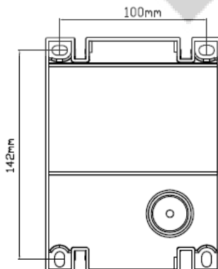
LAMP BASE FIXATION HOLES DIMENSIONS
