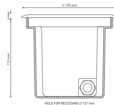
201018P HYDROFLOOR COMPACT SQUARE GU10
