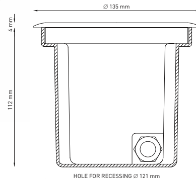
201015P HYDROFLOOR COMPACT SQUARE GU5.3
